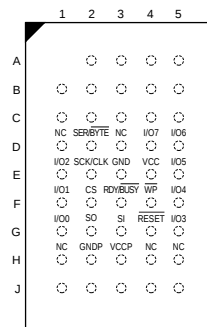
CBGA Top View
